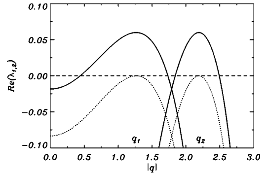
FIG. 4. Real part of the eigenvalues \lambda_{1,2} as a function of |\vec{q}| for the case of symmetric FH's coefficients. The solid lines correspond to F=1.06 and the dotted to criticality F=F_c=1 . Left branches correspond to \lambda_1 and the right ones to \lambda_2 . Here \gamma_{x,y}=\gamma'_{x,y}=1 and the values of the other parameters are the same as in Fig. 2. The most unstable modes q_1 and q_2 correspond to the maximum of each line. The level \text{Re}(\lambda_{1,2})=0 is also indicated as a dashed horizontal line as a reference.
